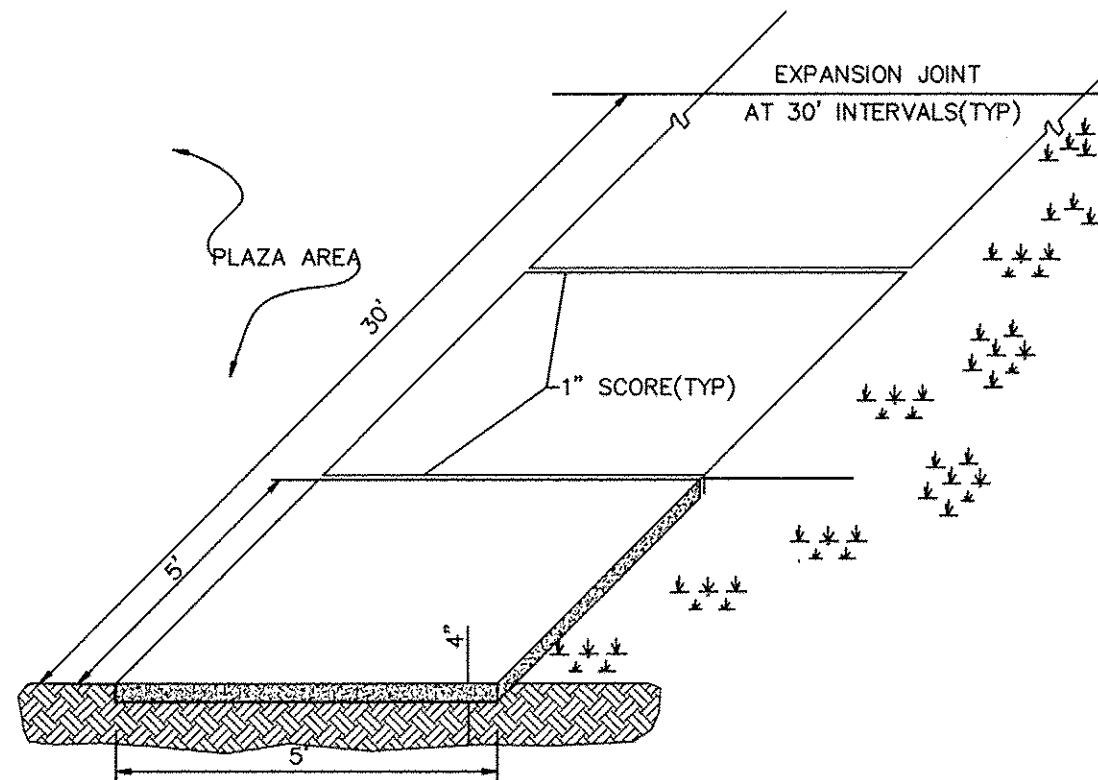
STANDARD SIDEWALK DETAIL SD 8-15 NOT TO SCALE
