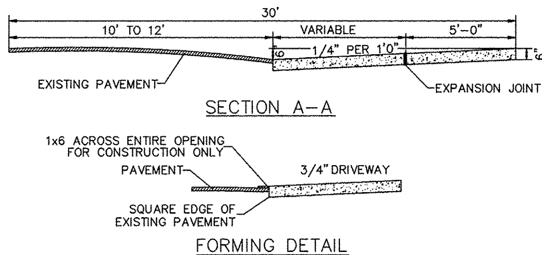
RESIDENTIAL DRIVEWAY STREETS WITH NO CURB SD 8-05 NOT TO SCALE
